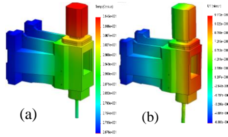
Figure 3. Thermal simulation results for the spindle system
