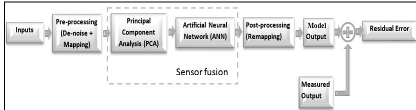
Figure 1. System architecture of the PCA-ANN based prediction model.
