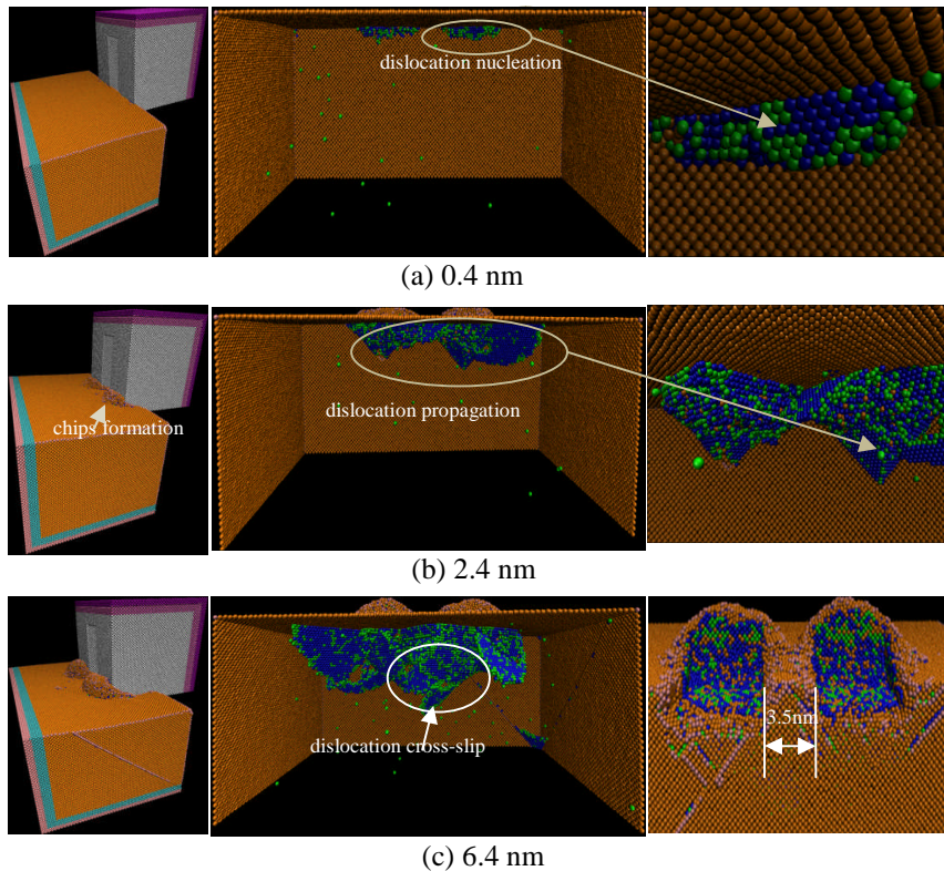
Figure 2: Snapshots of cutting process and dislocation evolution of workpiece at cutting distance of: (a) 0.4 nm, (b) 2.4 nm, and (c) 6.4 nm when a depth of cut is 1 nm.
