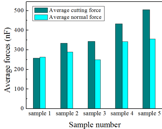
Figure 6: The average cutting forces under different depths of cut.
