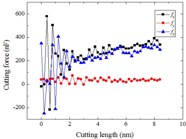
Figure 3: Force-displacement curves at the depth of cut of 1nm.
