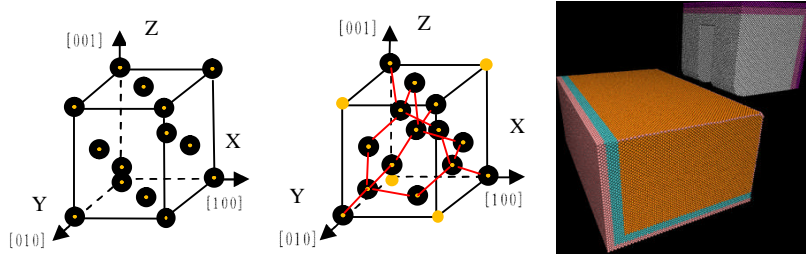
(a) FCC (b) Diamond crystal (c) Multi-tip tool cutting model Figure 1: Model of MD cutting simulation
