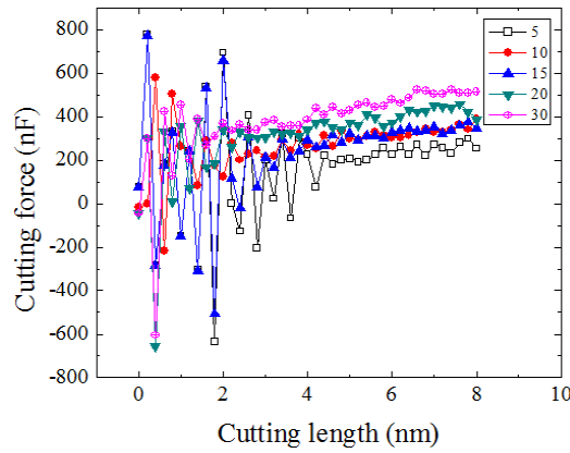
Figure 5: Force-displacement curves in the cutting process.
