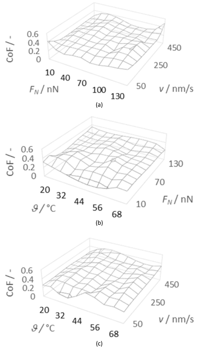
Figure 1. CoF values on a TiO 2 sample with fixed: \vartheta = 20^\circ\text{C} (a), v = 250\text{ nm/s} (b) and F_N = 50\text{ nN} (c).
