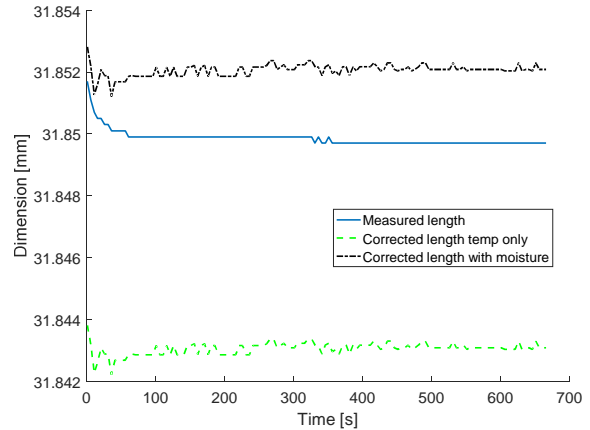
Figure 5. Results in terms of temperature and moisture uptake compensation for the ABS brick.
