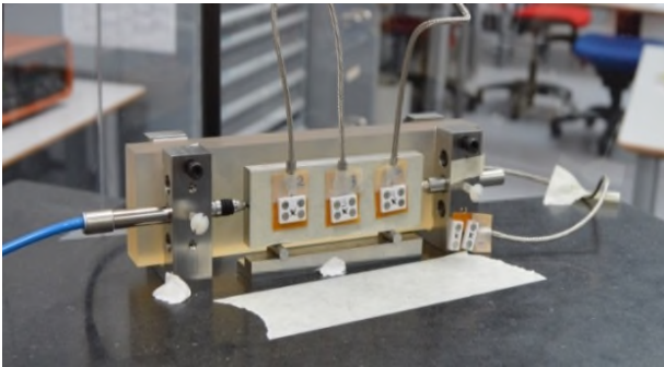
Figure 2. Setup for measuring the length of a steel gauge block, including temperature sensors.
