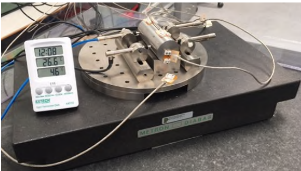
Figure 3. Setup for measuring the diameter of a steel cylinder in a non-controlled environment.
