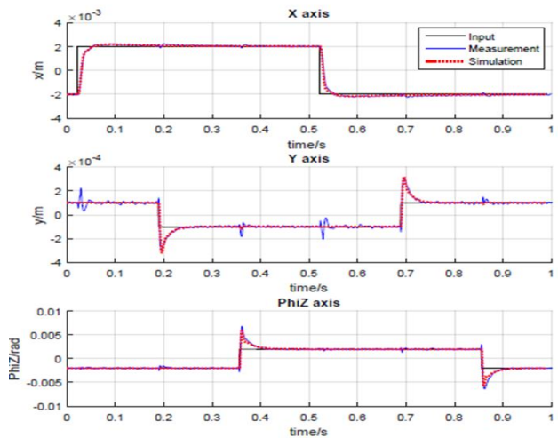
Figure 4. Step responses of the controlled axes
