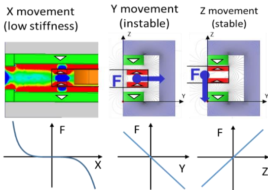
Figure 2. Schematics of the stable and unstable guidance axes
