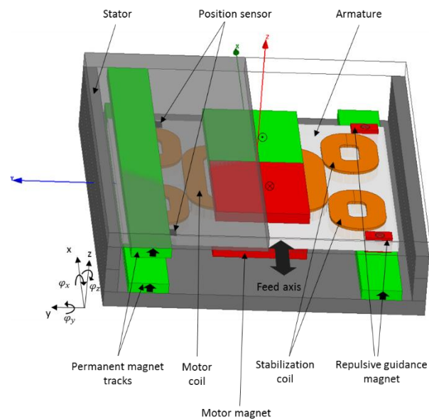
Figure 1. Motor and guidance concept
