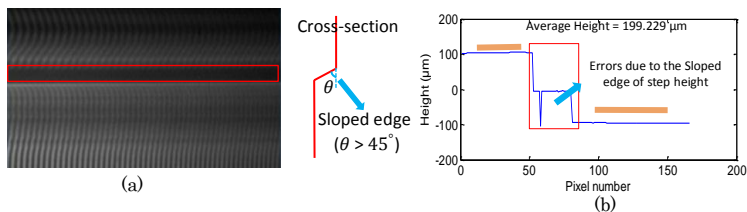
Figure 3: Measurement results (200 \mu\text{m} step): (a) interferogram, (b) 2D profile
