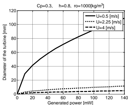
Figure 4. Power generated on a miniaturised turbine vs. river flow speed
