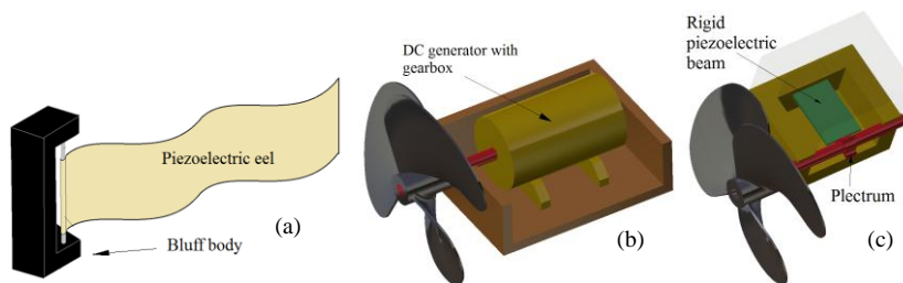
Figure 1: Considered energy harvesting solutions: piezoelectric eel (a), microturbine (b) and “plucked” piezoelectric beam (c)
