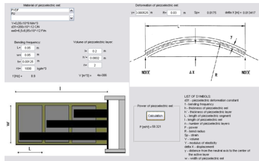
Figure 3. Matlab model of the piezoelectric eel
