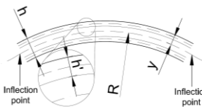
Figure 2. Bent section of the piezoelectric eel
