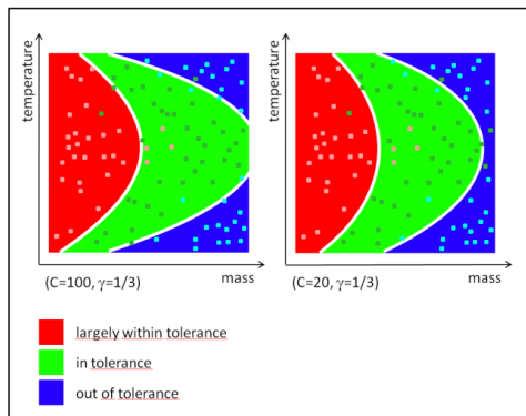
Figure 2: Example of SVM application to mass and temperature vectors
